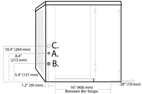
Air Cooled
